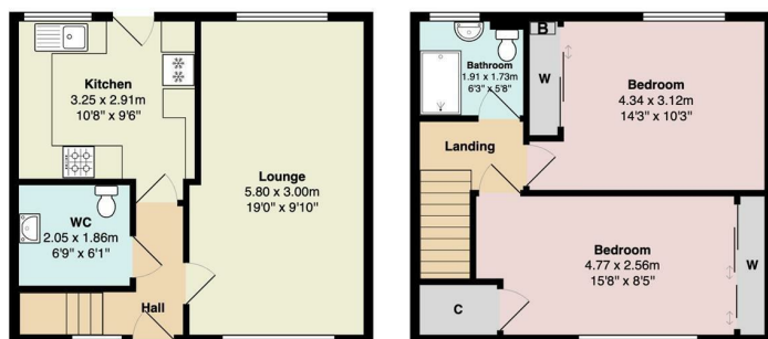
Ground Floor
